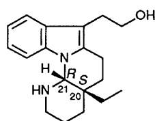
(20 S , 21 R ) - 1
