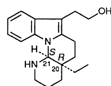
(20 R , 21 S ) - 1
